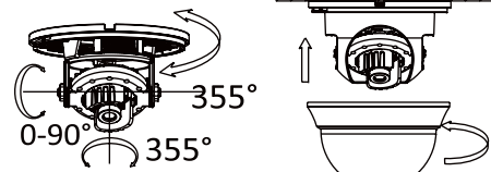
Figure 2-8 3-axis Adjustment & Lower Dome
